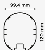
Profil vratnice Goal post section
