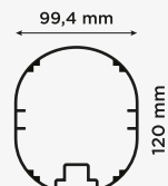
Profil vratnice Goal post section
