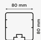
Profil vratnice Goal post section
