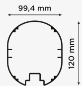
Profil vratnice Goal post section
