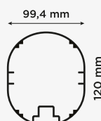
Profil vratnice Goal post section
