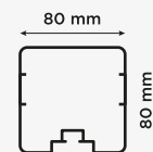
Profil vratnice Goal post section
