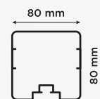
Profil vratnice (80x80) Goal post section (80x80)
